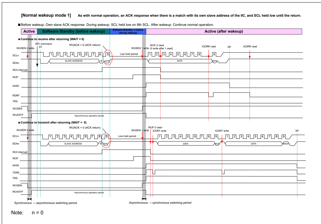
Figure 40.32 Timing of normal wakeup mode 1
