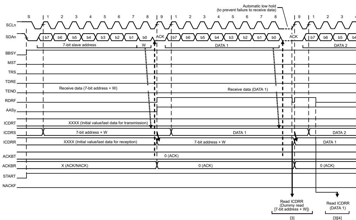
Figure 40.19 Slave receive operation timing (1) with 7-bit address format when RDRFS = 0
