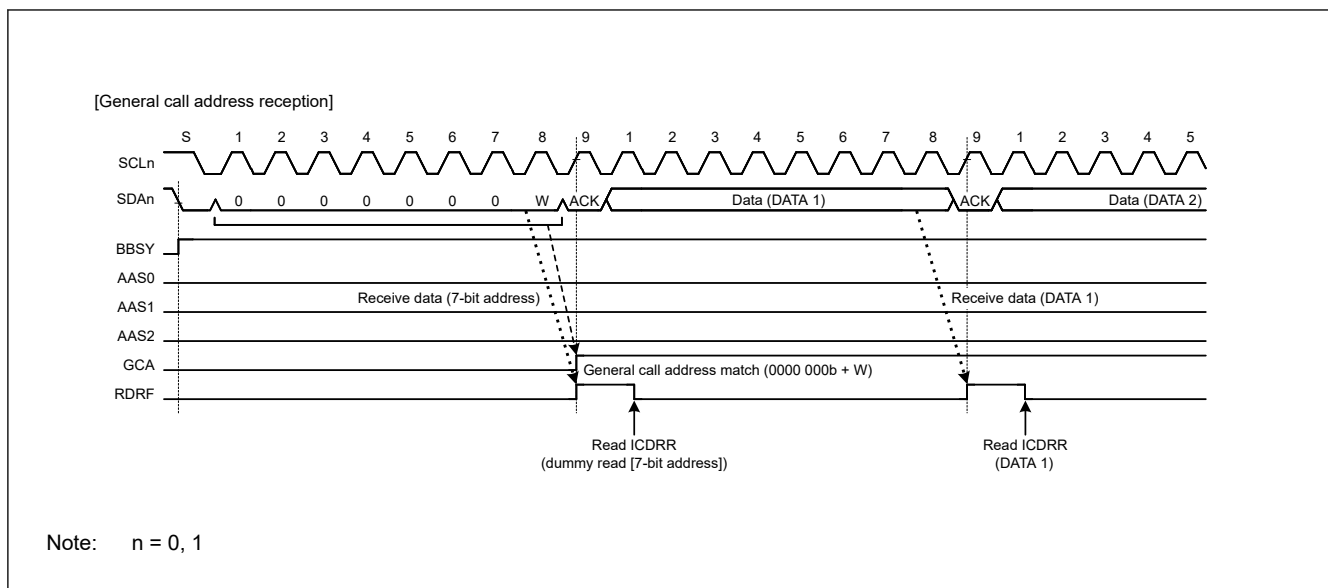
Figure 40.27 Timing of GCA flag setting during reception of general call address
